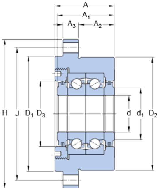
FBSA 206/DF Bearing 2D drawings and 3D CAD models
